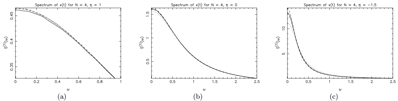
Fig. 8. Comparison of the equilibrium spectrum S^{(1)}(\omega) of x(t) for N = 4 as given by stochastic numerical simulations (solid line), exponential series extrapolation (dashed line), rational function extrapolation (dashed-dotted line), Lorentzian approximation (dotted line) for (a) \eta = 1 , (b) \eta = 0 , (c) \eta = -1.5 . Sampling error-bars at zero frequency are: (a) \Delta S = 0.002 , (b) \Delta S = 0.01 , (c) \Delta S = 0.1 .
