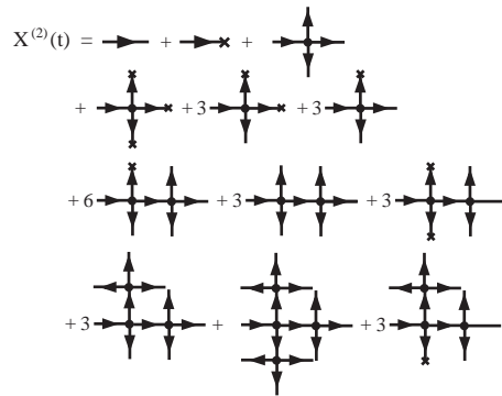
Fig. 2. Diagrammatic representation of the iterative solution of the cubic stochastic equation to second order.
